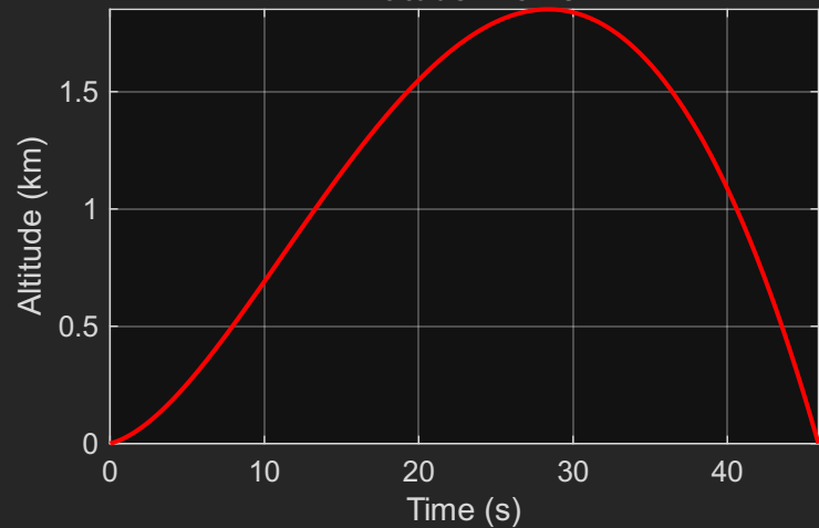
Altitude Profile
