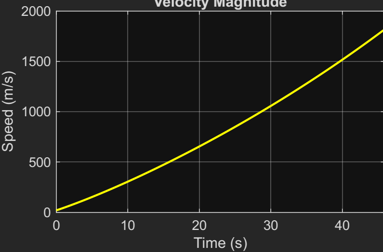
Velocity Magnitude
