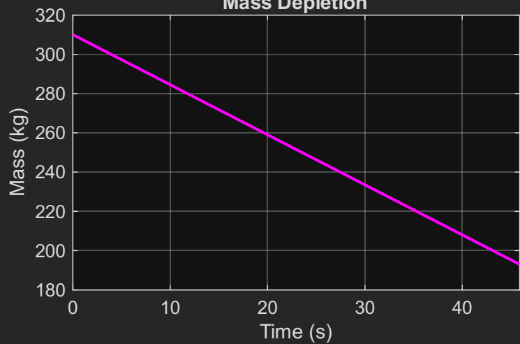
Mass Depletion
